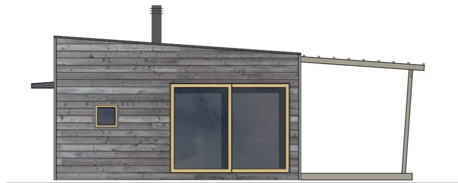
FASAD A
